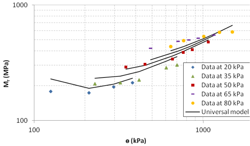
Figure 5 Resilient Modulus vs. bulk stress for test data and Universal model
