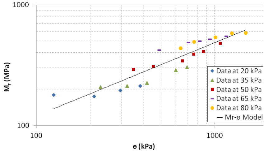
Figure 4 Resilient Modulus vs. bulk stress for test data and Mr- \theta model
