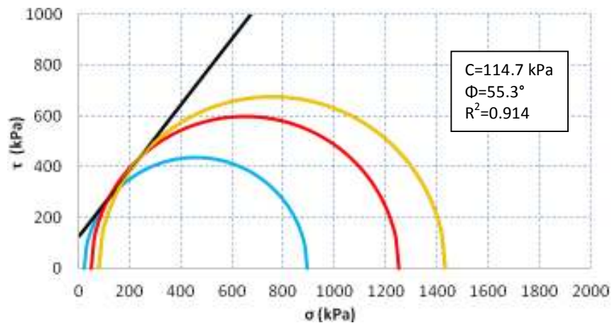
Figure 3 Mohr-Coulomb circles of G1 material at 100 per cent of DOC and 80 per cent of saturation
