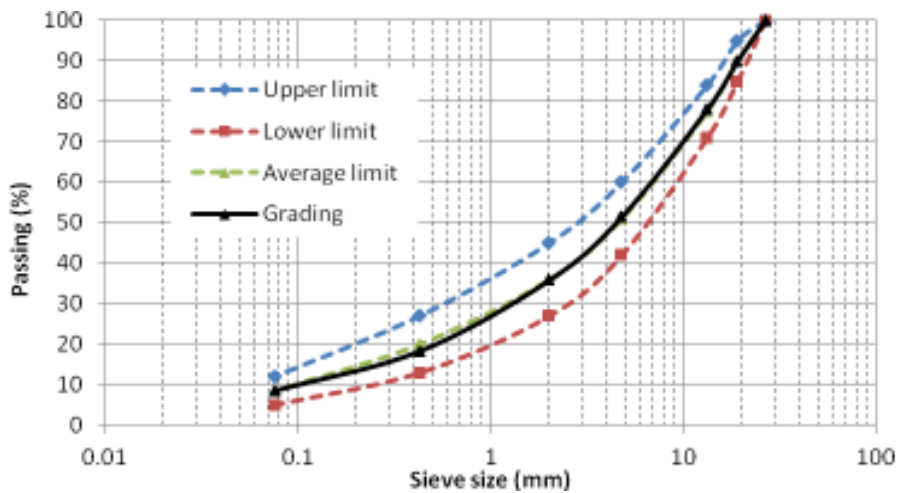
Figure 1 Grading curve of G1 material
