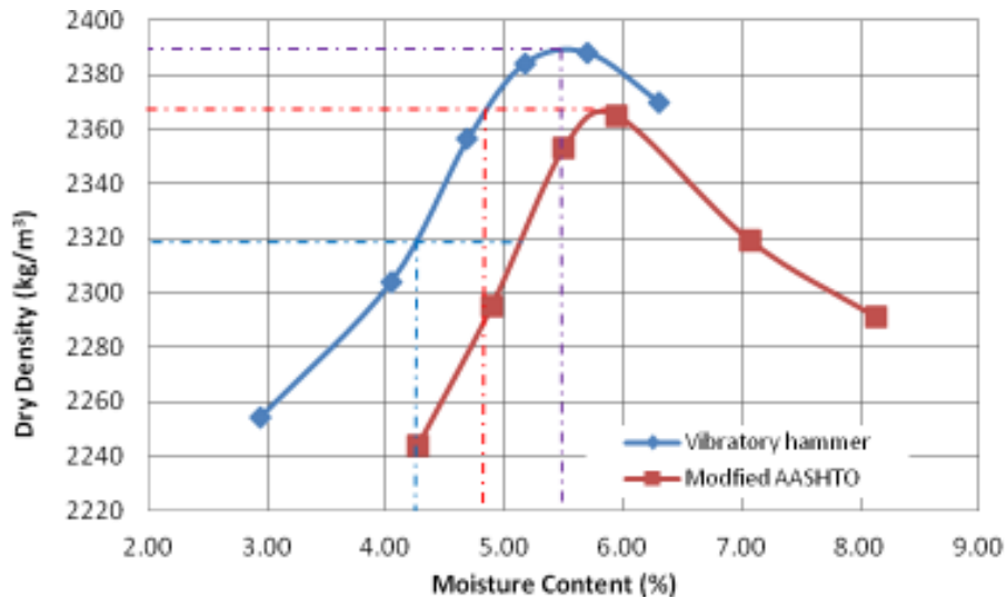
Figure 2 Determination of OMC and MDD for G1 material
