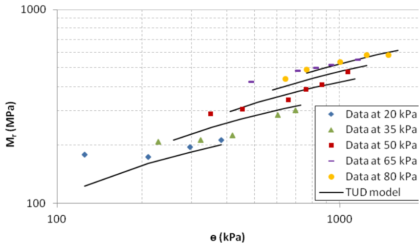
Figure 6 Resilient Modulus vs. bulk stress for test data and TUD model
