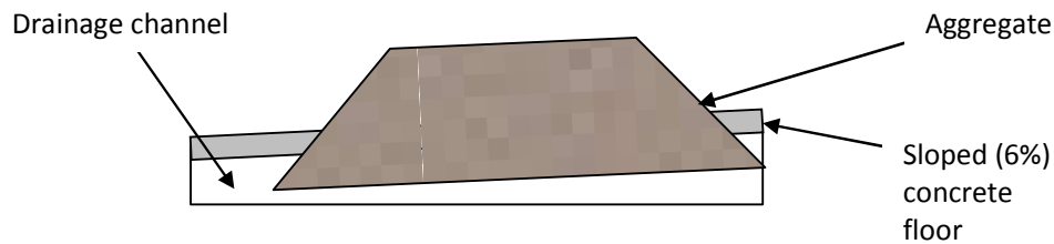
Figure 1: Aggregate placement under roof to effectively drain moisture
