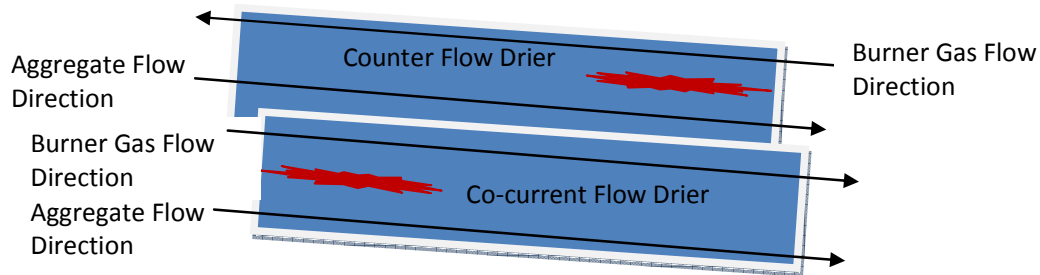
Figure 2: Drier aggregate/burner gas flow direction arrangements
